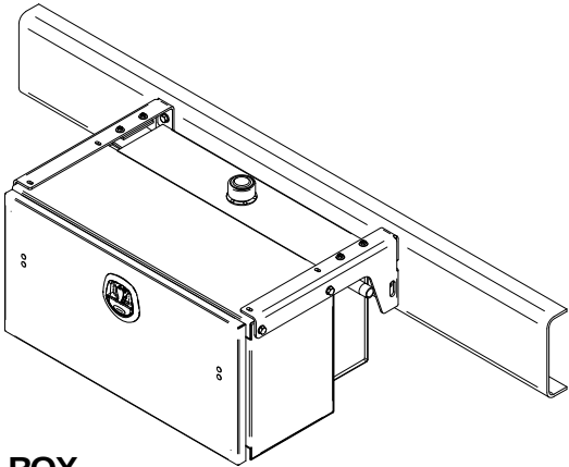
36" TOOLBOX w/ HYDRAULIC RESERVOIR
