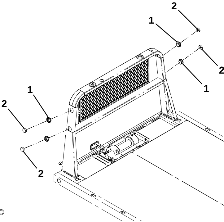
FOR 45", 50" & 57" HEADBOARDS
