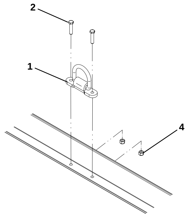
STEEL DECK
