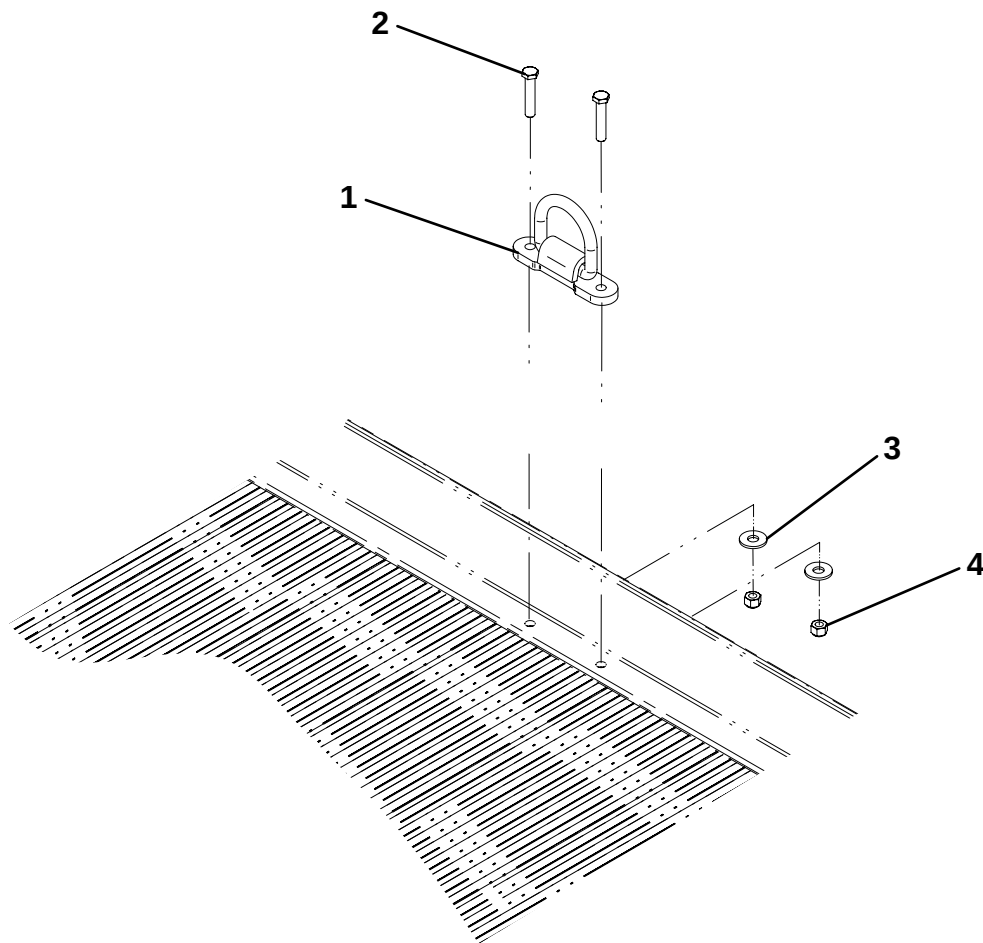
ALUMINUM DECK
