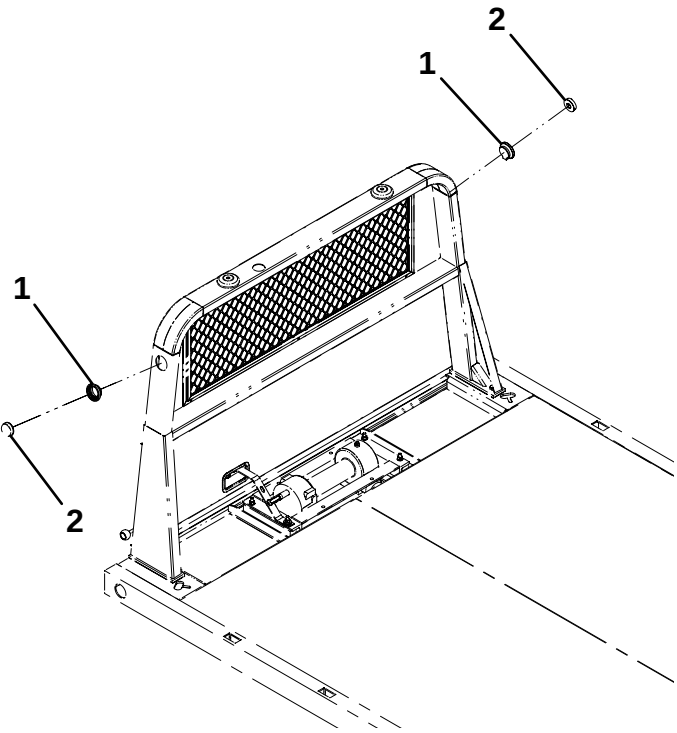
FOR 36" & 40" HEADBOARDS
